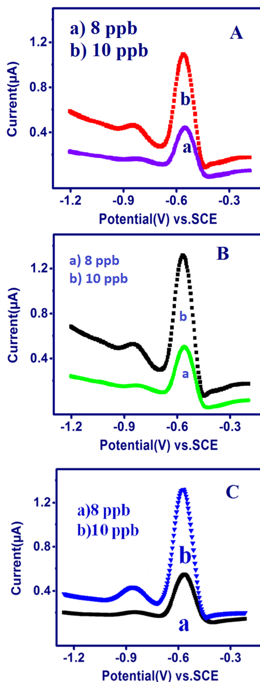
Fig. 8 SWASV of the TSAB/MWCNT in pH 5.5 ABS containing a 10 ppb mixture of \text{Pb}^{2+} and \text{Cd}^{2+} at an Eacc of -1.2 V and Tacc of 240 s in a few environmental samples: honey (A), raw milk (B) and groundnut shell (C).
