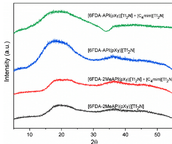
Fig. 14 XRD profiles of 6FDA C(2)–H and C(2)–Me, both neat and composite, Pls.
