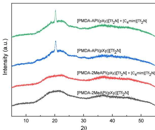
Fig. 13 XRD profiles of PMDA C(2)–H and C(2)–Me, both neat and composite PI-ionenes.
