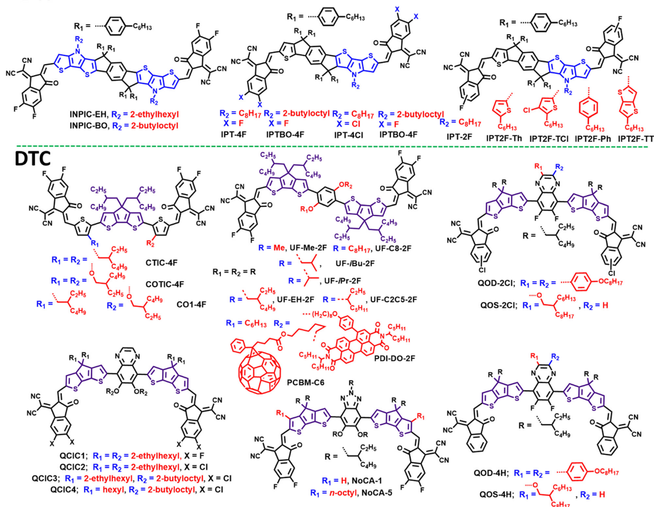
Fig. 10 Chemical structures of DTP- and DTC-based SMAs with different side chains.
