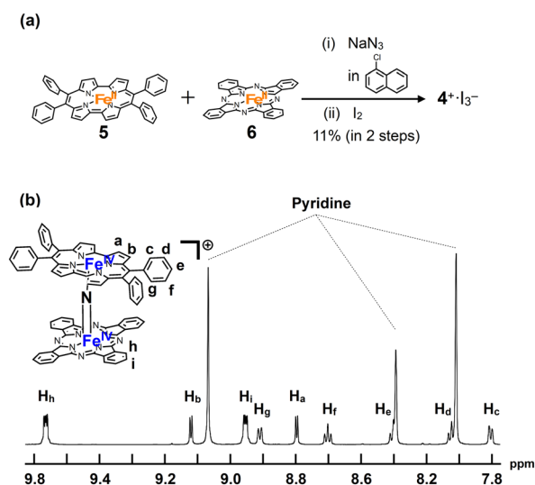
Fig. 2 (a) Synthesis of a monocationic heterodimer 4 + ·I 3 − . (b) 1 H-NMR spectrum of 4 + ·I 3 − in pyridine- d 5 .
