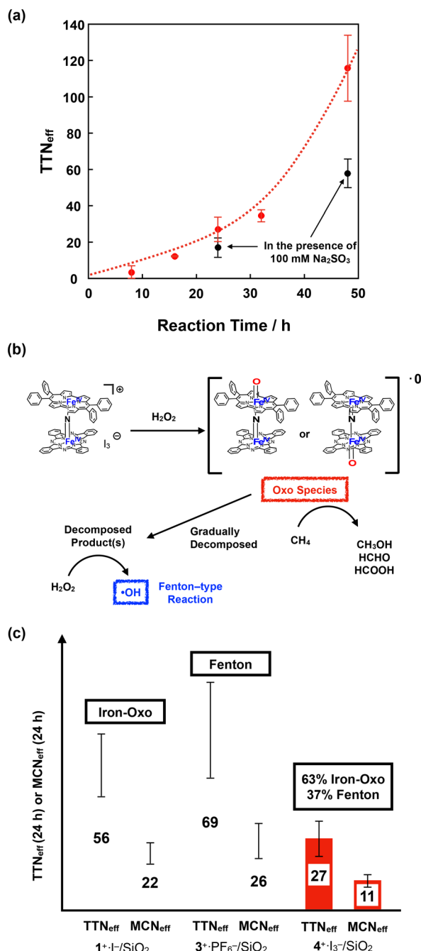
Fig. 9 (a) Time dependence of TTN_{eff} for CH_4 oxidation by 4^+\cdot I_3^- in the absence (red circle) and presence (black circle) of 100 mM Na_2SO_3 . Error bars indicate standard deviations of three independent oxidation reactions. (b) Proposed reaction mechanism for the CH_4 oxidation by 4^+\cdot I_3^- . (c) Comparison of TTN_{eff} and MCN_{eff} for the CH_4 oxidation for 24 h by 1^+\cdot I^- , 3^+\cdot PF_6^- , and 4^+\cdot I_3^- .
