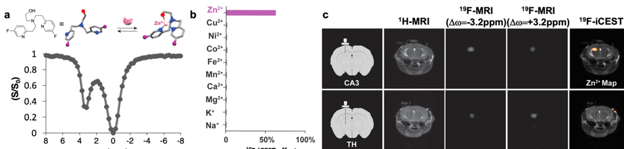
Fig. 7 19 F-iCEST for mapping labile Zn 2+ pools. (a) The molecular structure of the ultimate 19 F-iCEST probe designed for mapping labile Zn 2+ and the obtained 19 F-iCEST effect (Δω = 3.2 ppm) of 3 mM probe and 30 μM Zn 2+ . (b) 19 F-iCEST effect (Δω = 3.2 ppm) of 3 mM probe and 30 μM s-block (Na + , K + , Mg 2+ , Ca 2+ ) and d-block (Mn 2+ , Fe 2+ , Co 2+ , Ni 2+ , Cu 2+ , Zn 2+ ) metal ions obtained at 37 °C using a 9.4 T NMR spectrometer. (c) In vivo 19 F-iCEST maps of labile Zn 2+ pools in the mouse brain. The results are shown for two regions of the brain: CA3 in the hippocampus (zinc-rich ROI, upper row) or the thalamus (TH, zinc-poor ROI, lower row). From left to right are the schematic illustrations of the setup used to deliver a zinc-responsive probe to either CA3 or TH, 1 H-MRI, 19 F-MRI obtained with saturation pulse applied "off-resonance" (Δω = -3.2 ppm), 19 F-MRI obtained with saturation pulse applied "on resonance" (Δω = +3.2 ppm), the 19 F-iCEST map (Zn 2+ map) obtained from subtracting 19 F-MRI S +3.2 ppm from 19 F-MRI S -3.2 ppm overlaid on the 1 H-MRI. Modified with permission from ref. 76.
