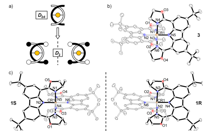
Fig. 1 (a) Illustration of the chiral structures. Crystal structures of complexes (c) 1S/1R and (b) 3 , drawn in 50% probability ellipsoids with H-atoms, counter-ions and solvate molecules omitted for clarity.
