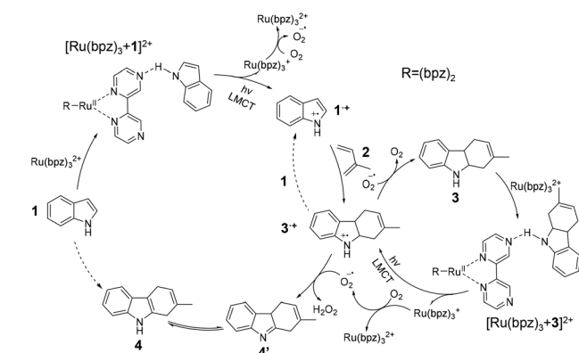
Fig. 5 Possible mechanism of the photocatalytic indole cation-radical cyclization reaction in confined space. 1 – 4 : reactant, intermediates and product detected by in situ nano-electrospray MS.
