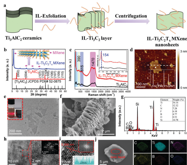
Fig. 1 Synthesis and characterization of IL-Ti 3 C 2 T x MXene nanosheets. (a) Schematic illustration of the synthesis of IL-Ti 3 C 2 T x MXene nanosheets. (b) XRD patterns, (c) Raman spectra, and (d) AFM image of IL-Ti 3 C 2 T x MXene. (e) TEM images of IL-Ti 3 C 2 T x MXene. The inset shows a photograph of IL-Ti 3 C 2 T x MXene nanosheets dispersed in water. (f) SEM images and EDS spectra (g) of IL-Ti 3 C 2 T x MXene. (h) HRTEM image of overall and partial magnification (left) and the corresponding selected area electron diffraction (SAED) pattern of the IL-Ti 3 C 2 T x MXene (right). (i) HRTEM images and corresponding FFT patterns of the IL-Ti 3 C 2 T x MXene. The insets show diagrams of the lattice spacing. (j) SEM elemental mapping of IL-Ti 3 C 2 T x MXene.
