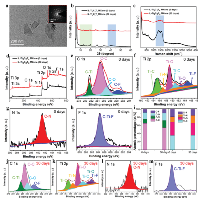
Fig. 2 Stability of IL-Ti 3 C 2 T x MXene nanosheets. (a) TEM images of IL-Ti 3 C 2 T x MXene after 30 days of storage. The inset shows a corresponding FFT pattern. (b) XRD patterns and (c) Raman spectra of the IL-Ti 3 C 2 T x MXene before and after one month of storage. XPS spectra and fitting analysis of IL-Ti 3 C 2 T x MXene nanosheets for (d) total survey, (e) C1s, (f) Ti 2p, (g) N 1s, and (h) F1s, respectively. (i) The histogram of the integral area graph from the XPS peak fitting results of the Ti 2p and C 1s regions of IL-Ti 3 C 2 T x MXene. (j–m) XPS spectra of IL-Ti 3 C 2 T x MXene after one month of storage.
