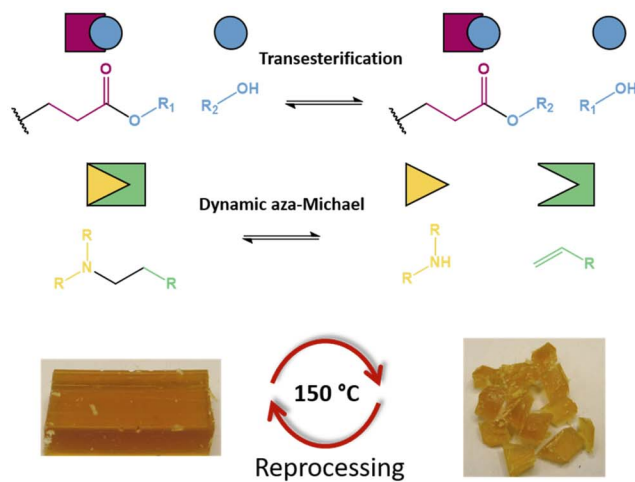
Fig. 6 Schematic representations of BAE-F-OH, BAE-F and BAE-OH associated with their respective exchange reactions and reprocessing conditions.
