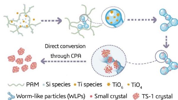
Fig. 6 Scheme of the putative crystallization pathway of TS-1 in the presence of PAM.
