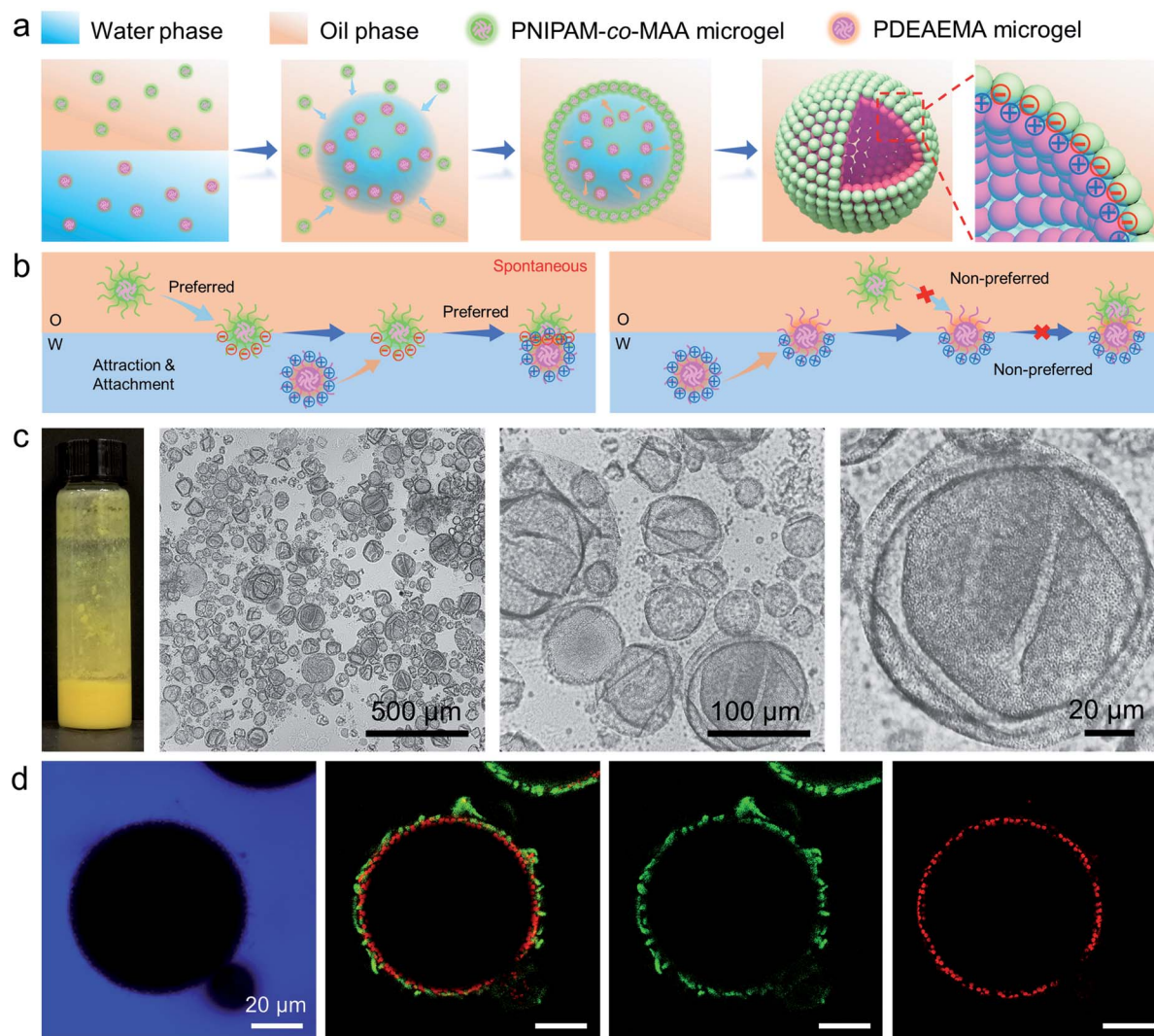
Fig. 3 (a) Schematic illustration of the formation process and interfacial bilayer structure of the microgelosome constructed from oppositely charged binary microgels. (b) Proposed stabilization mechanism of the microgel bilayer at the interface, with oppositely charged microgels dispersed in different phases. (c) Photographs, optical microscopy images and (d) CLSM images of non-covalent microgelosomes during solvent evaporation, stabilized by 0.5 wt% PNIPAM-co-MAA microgels (green) in the oil phase and 0.5 wt% PDEAEMA microgels (red) in the water phase. The microgelosomes composed of a microgel bilayer structure with numerous wrinkles appeared on the surface.
