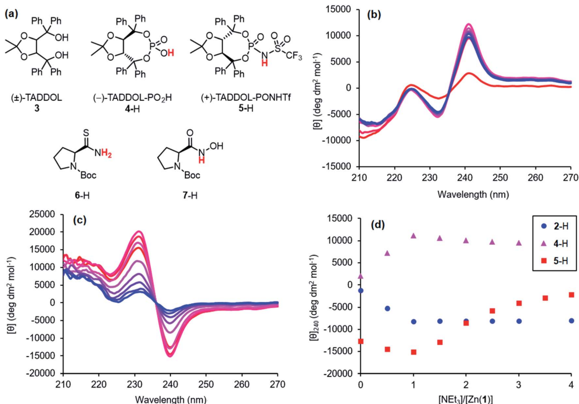
Fig. 3 (a) Structures of 3 and ligands 4 – 7 ; CD spectra of \text{Zn}(\mathbf{1}) \cdot 2\text{ClO}_4 ( c_0 = 0.25 mM) with (b) 4 -H (1 eq.) or (c) 5 -H (1 eq.) in MeCN with addition of \text{NEt}_3 (0.0 \rightarrow 4.0 eq.) in 0.5 eq. increments; (d) molar ellipticities at 240 nm of \text{Zn}(\mathbf{1}) \cdot 2\text{ClO}_4 ( c_0 = 0.25 mM) and 2 -H, 4 -H or 5 -H (1 eq.) with addition of \text{NEt}_3 .
