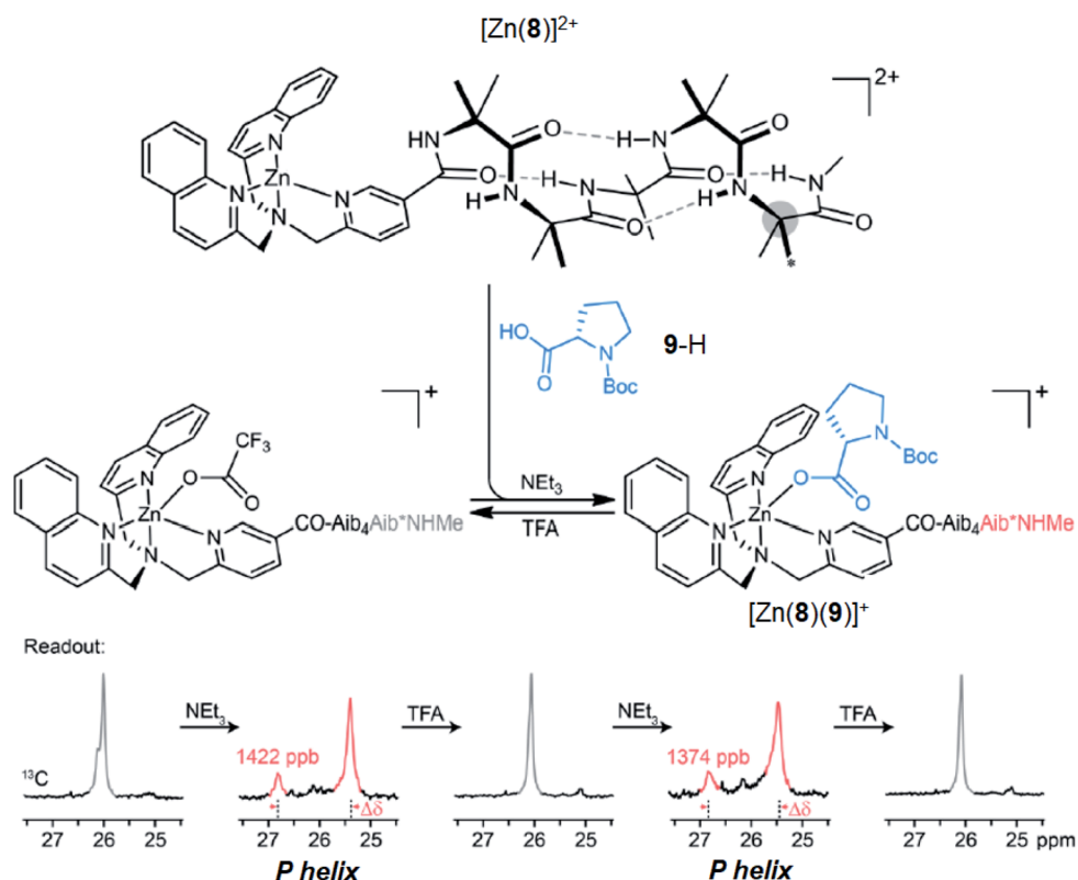
Fig. 10 pH-induced binding of 9-H with complex [\text{Zn}(\mathbf{8})]^{2+} ( c_0 = 12.1 mM) with alternating addition of \text{NEt}_3 and TFA in 1.2 eq. increments, monitored by 13 C NMR of the terminal Aib*NHMe reporter.
