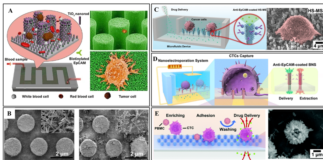
Fig. 4 3D micro-/nanostructure integrated microfluidic devices. (A) Vertical growth of \text{TiO}_2 nanorods on silicon nanopillars for immunoaffinity capture. Reprinted with permission from ref. 2. Copyright (2017) Springer Nature. (B) ZnO coated PDMS microrod array from the first synthesis cycle (left) and the second cycle (right). Reprinted with permission from ref. 6. Copyright (2018) American Chemical Society. (C) Hierarchical spiky microstraw array-integrated microfluidic device for immunoaffinity capture and in situ chemical manipulation. Reprinted with permission from ref. 16. Copyright (2019) John Wiley and Sons. (D) Branched nanostraw-electroporation platform for immunoaffinity capture, downstream regulation and monitoring intracellular activities. Reprinted with permission from ref. 24. Copyright (2019) American Chemical Society. (E) Hybrid \text{TiO}_2/\text{ZnO} branched microtube array for antibody-free separation and in situ regulation. Reprinted with permission from ref. 30. Copyright (2020) Royal Society of Chemistry.
