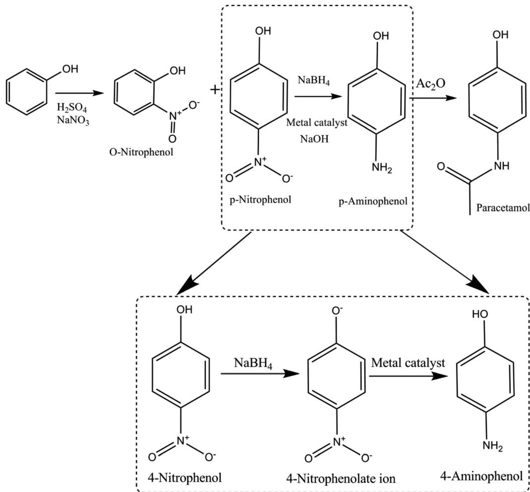
Fig. 2 Schematic representing the history of 4-nitrophenol acquired during the production of paracetamol from phenol as an intermediate product.
