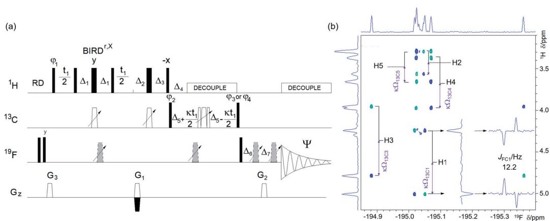
Fig. 6 (a) Pulse sequence of the (3, 2)D ^1\text{H} ^{13}\text{C} ^{19}\text{F} correlation experiment. For explanation of symbols used for pulses see Experimental. The NMR parameters used are given in Table S1.† The delays were as follows: d_2 = 0.25/{}^1J_{\text{HC}} ; d_3 = 0.5/{}^1J_{\text{HC}} ; d_4 = 0.25/{}^nJ_{\text{FC}} ; d_6 = \text{cnst}1/{}^1J_{\text{HC}} , where \text{cnst}1 = 0.5 for CH and 0.25 for \text{CH}_2 groups; \Delta_1 = d_3 - p14/2 ; \Delta_2 = d_2 - p14/2 - p16 - d16 ; \Delta_3 = d_2 - p14/2 - 2t_1(0) ; \Delta_4 = d_6 ; \Delta_5 = d_4 ; \Delta_6 = p16 + d16 - (2/\pi)p1 + 4 \mu\text{s} ; \Delta_7 = p16 + d16 + 4 \mu\text{s} , where p16 and d16 are the PFG length and the recovery time, respectively. The gradient strengths were as follows: G_1 = 40\% ; G_2 = 42.51\% ; G_3 = 13\% . The following phase cycling was used: \varphi_1 = y, -y ; \varphi_2 = 4x, 4(-x) ; \varphi_3 = 2x, 2(-x) ; \varphi_4 = 2y, 2(-y) ; \Psi = x, 2(-x), x, -x, 2x, -x . The echo-antiecho protocol was used with G_1 changing sign between real and imaginary increments. Phases \varphi_1 and \Psi were incremented by 180^\circ together with the sign change. Two interleaved experiments were acquired applying either the \varphi_3 or \varphi_4 phase to the last 90^\circ ^{13}\text{C} pulse, (b) an F_1 antiphase (3, 2)D ^1\text{H} ^{13}\text{C} ^{19}\text{F} spectra of 1 acquired using the pulse sequence shown in (a) showing the cross peaks of the \beta -anomer of 1 . Positive and negative cross peaks are shown in blue and turquoise, respectively. The insets contain vertical and horizontal traces through the H1, F cross peaks. The ^1\text{H} chemical shift of protons directly attached to ^{13}\text{C} atoms and the associated \kappa\Omega_{^{13}\text{C}} frequencies are indicated. Antiphase doublets in F_2 show ^nJ_{\text{FC}} coupling constants. Horizontal and vertical internal projections are shown on the top and along the left side of all spectra, respectively. The editing process that simplifies this spectrum is explained in the text and shown in Fig. S5.†
