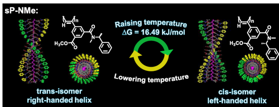
Fig. 33 Schematic depiction of the possible 3D helical models and the conformations of pendants for poly(( S )-3-methoxycarbonyl-5-( N -methyl- N -( S )-(1-phenylethyl)carbamoyl)phenylacetylene) in CHCl 3 . Adapted from ref. 158 Copyright 2021 American Chemical Society.
