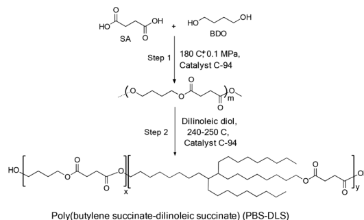
Scheme 38 Synthesis of PBS-DLS copolymer.
