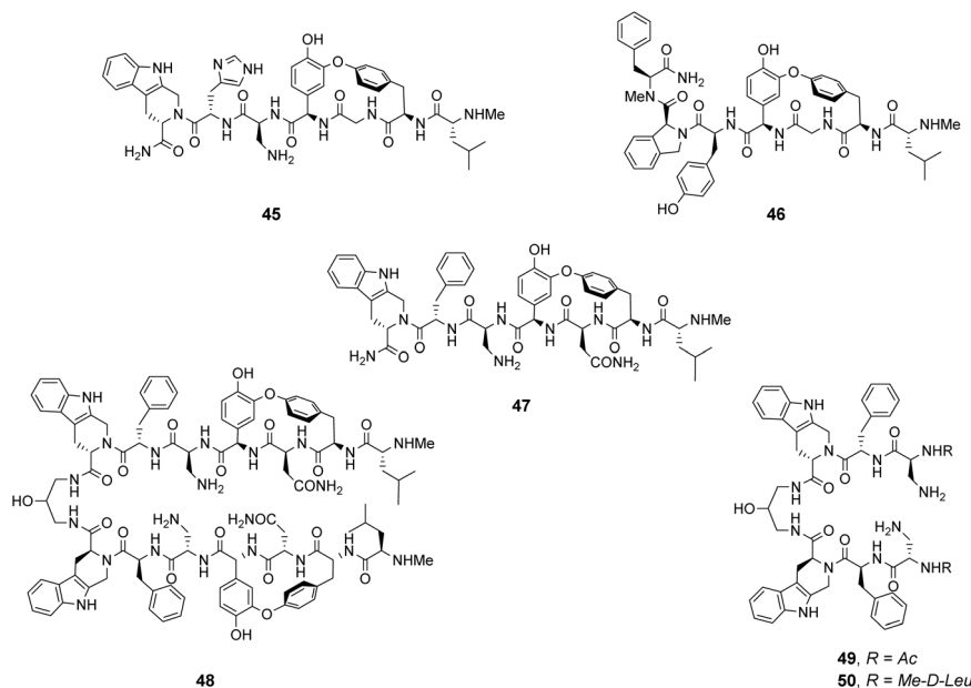
Fig. 17 Combinatorial receptors 45–47 mimicking vancomycin's DE-ring. Dimer 48 was based on the most biologically active library member. Two control compounds 49 and 50 were used to interrogate the mechanism of action.
