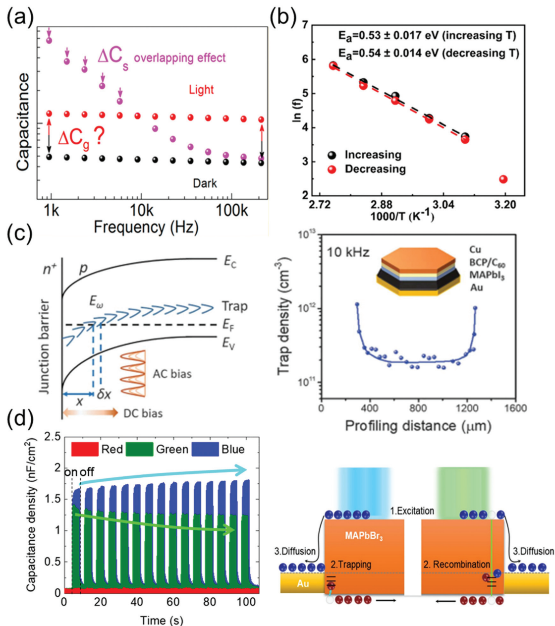
Fig. 12 (a) C - F curve of an MAPbBr 3 single-crystal device under dark conditions and under illumination. Reproduced with permission. 111 Copyright 2018, ACS. (b) Arrhenius plots of the inflection frequencies vs. 1000/T ( \ln(f_0) vs. 1000/T ) with the increasing and decreasing temperature of the MAPbBr 3 single crystal. E_{act} is the activation energy for the traps. Reproduced with permission. 113 Copyright 2020, ACS. (c) DLCP technique. (left) Schematic of band bending of a p-type semiconductor with deep trap states in an n + -p junction. (right) The inset shows the device structure. Reproduced with permission. 110 Copyright 2020, AAAS. (d) Time-dependent photocapacitance under red, green, and blue light illumination, and schematic of the carrier transport mechanism for MAPbBr 3 under blue and green light illumination. Reproduced with permission. 112 Copyright 2021, IOP Publishing.
