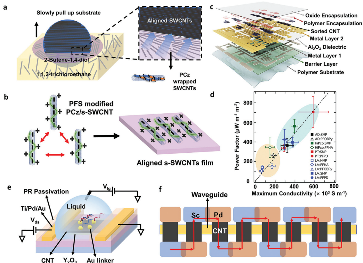
Fig. 6 (a) Schematic images of DLSA procedure to assemble aligned-SWCNT arrays on a 4-inch wafer. The purple layer is formed by 2-butene-1,4-diol ( \text{C}_4\text{H}_8\text{O}_2 ). As the wafer is slowly pulled out, the possible hydrogen bonds between polymers and \text{C}_4\text{H}_8\text{O}_2 allowed the confined on the interface between two insoluble solvents and assembled onto the wafer surface along the contact line. (b) Schematic illustration of a positively charged conjugated molecule, proflavine hemisulfate (PFS), modifying the surface of PCz wrapped s-SWCNTs. The positive charges can prevent the aggregation of s-SWCNTs during alignment. (c) Layer structure of the digital and analog circuits build on a flexible substrate. Reproduced with permission. 3 Copyright 2019, Springer Nature. (d) Relationship between maximum thermoelectric (TE) power factor (optimally doped network) and the maximum conductivity (fully doped network) for different types of sorted s-SWCNT networks. The maximum conductivity and TE power factor for s-SWCNT networks using removable polymers (SMP, PFPD, blue oval) are larger than the values for s-SWCNT networks sorted with non-removable polymers (PFOBPy, PFHA, orange oval). Among them, plasma-torch s-SWCNT network with PFPD exhibited the highest TE power factor. Reproduced with permission. 89 Copyright 2017, Royal Society of Chemistry. (e) Schematic diagram of a carbon nanotube floating-gate FET biosensor. The ultrathin high-k \text{Y}_2\text{O}_3 passivation layer is helpful to amplify response and improve sensitivity. (f) Schematic diagram of a series carbon nanotube photo-detector device contains eight cells. Red arrows represent a current direction at forward bias. The cells are connected by a pair of overlapping Sc and Pd electrodes.
