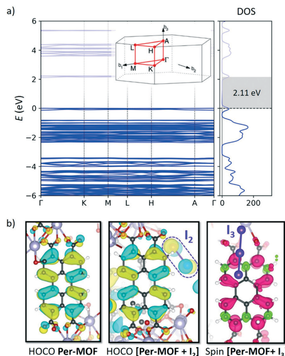
Fig. 4 a) Band structure and density of states (DOS) calculated at the HSE06 level for the full k -path of the first Brillouin zone of P\bar{3} space group in Per-MOF . The Fermi level was set to the valence band maximum. b) Highest-occupied crystal orbital (HOCO) calculated for evacuated Per-MOF and iodine-doped [ Per-MOF + I 2 ], and spin density calculated for [ Per-MOF + I 3 ].
