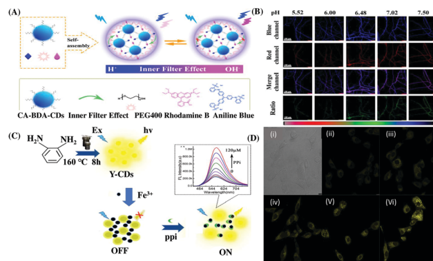
Fig. 4 (A) Schematic diagram of the preparation of RhB-AB-CDs and their sensing mechanism at acidic and basic pH. (B) Confocal fluorescence images of Pholiota adiposa mycelia stained by RhB-AB-CDs at different pH values. Adopted with permission from ref. 66. (C) Fluorescence response of y-CDs- \text{Fe}^{3+} in the presence of PPI. (D) Confocal microscopy (i) bright-field and (ii) dark-field images of A-549 cells co-incubated with y-CDs and \text{Fe}^{3+} , and (iii and vi) images of co-stained A-549 cells using the y-CDs- \text{Fe}^{3+} ensemble with different concentrations of PPI. Adopted with permission from ref. 73.
