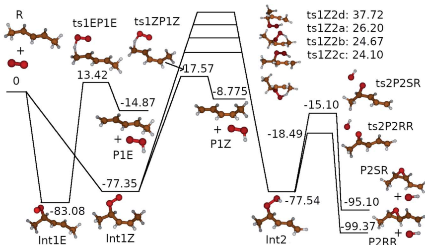
Fig. 7 The zero-Kelvin reaction enthalpy ( \Delta_r H_0^\ominus ) profile used in the master equation simulations. The energies are in kJ mol -1 .
