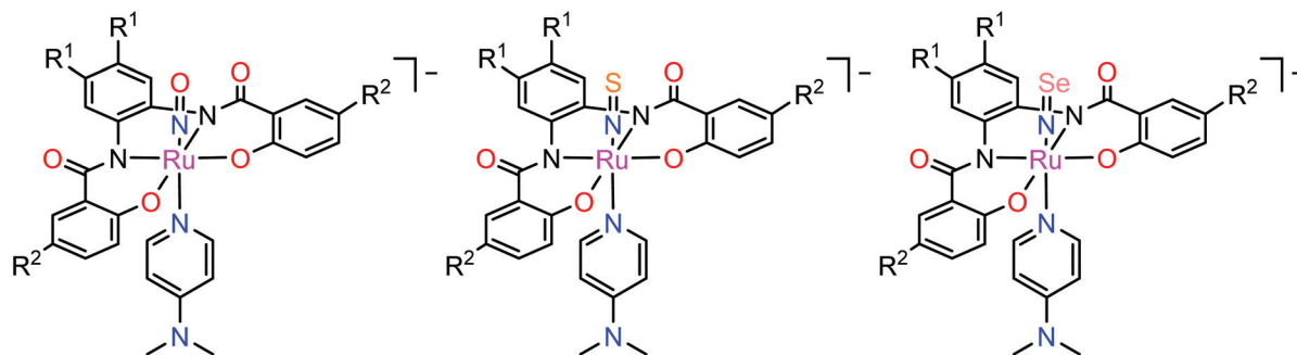
Chart 1 The line drawings of the complex anions [\text{Ph}_4\text{P}][\text{Ru}(\text{NE})(\text{hybeb}^{\text{R1,R2}})(\text{DMAP})] ( \text{R}^1 = \text{R}^2 = \text{Cl} , \text{R}^1 = \text{H} , \text{R}^2 = \text{CF}_3 , \text{R}^1 = \text{Cl} , \text{R}^2 = \text{CF}_3 ; \text{E} = \text{O} , \text{S} , \text{Se} ) isolated as tetraphenylphosphonium salts.
