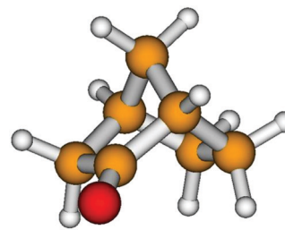
Fig. 1 Sketch of the (+)-(1S,4R)-norcamphor molecule.
