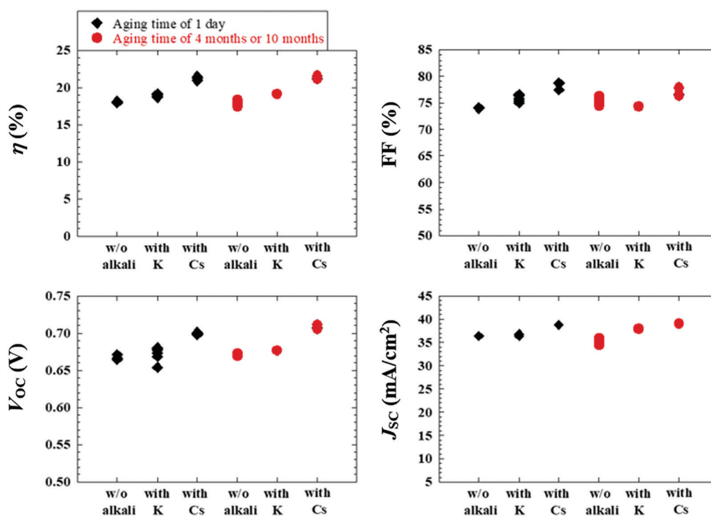
Fig. 17 Photovoltaic performance of the CdS-buffered CIGS Se solar cells using aged CIGS Se absorbers for aging times of 1 day, as well as 4 months or 10 months, where the absorbers were processed with and without the alkali (Cs or K) treatment.
