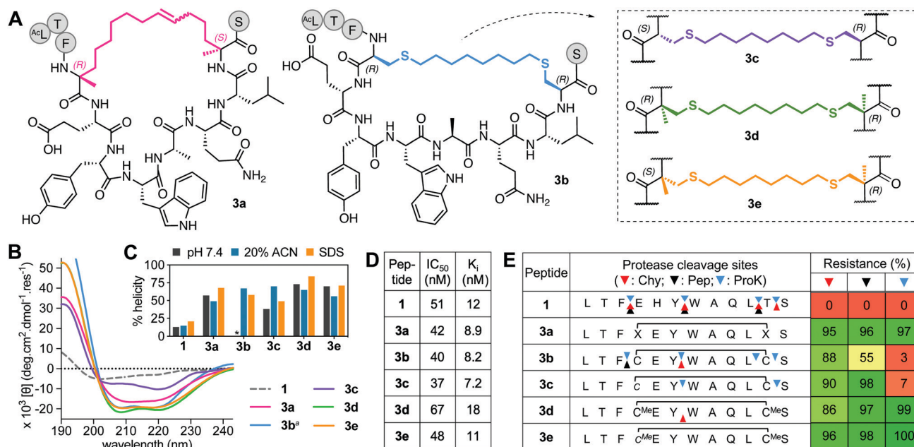
Fig. 3 A. Structures of aliphatic ( i \rightarrow i + 7 )-crosslinked peptides 3a–e . B. CD spectra for 3a–e vs. 1 (50 \mu M) in 10 mM phosphate buffer (pH 7.4, 22 °C) except 3b a in 20% ACN. C. Percent helicity calculated from CD spectra ( \theta_{220} ) in 10 mM phosphate buffer, 20% ACN or 20 mM SDS buffer (* not helical). D. IC 50 is mean peptide concentration to inhibit 50% binding of 1-FITC (10 nM) to hDM2 (25 nM) measured by FP. pIC 50 \pm SEM values are reported in Fig. S1 (ESI † ). Binding affinity (K i ) calculated from IC 50 values. E. Heatmap indicating percent peptide intact after 2 h incubation with chymotrypsin (Chy), pepsin (Pep) or proteinase K (ProK) at 22 °C and pH 8 or 2 (Pep only), measured by LCMS. Arrows point to respective cleavage sites as revealed by LCMS analysis of the cleaved fragments.
