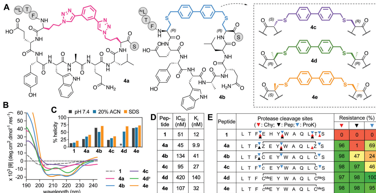
Fig. 4 A. Structures of aromatic ( i \rightarrow i + 7 )-crosslinked peptides 4a–e . B. CD spectra for 4a–e vs. 1 (50 \mu M) in 10 mM phosphate buffer (pH 7.4, 22 °C), except 4d a in 20% ACN. C. Percent helicity calculated from CD spectra ( \theta_{220} ) in 10 mM phosphate buffer, 20% ACN or 20 mM SDS buffer (* not helical, Fig. S2, ESI † ). D. IC 50 = mean peptide concentration to inhibit 50% binding of 1-FITC (10 nM) to hDM2 (25 nM) measured by FP. pIC 50 \pm SEM values are reported in Fig. S1, ESI † . Binding affinity (K i ) calculated from IC 50 values. E. Heatmap indicating percent peptide intact after 2 h incubation with chymotrypsin (Chy), pepsin (Pep) or proteinase K (ProK) at 22 °C at pH 8 or 2 (Pep only), measured by LCMS. Arrows show cleavage sites revealed by LCMS of the cleaved fragments.
