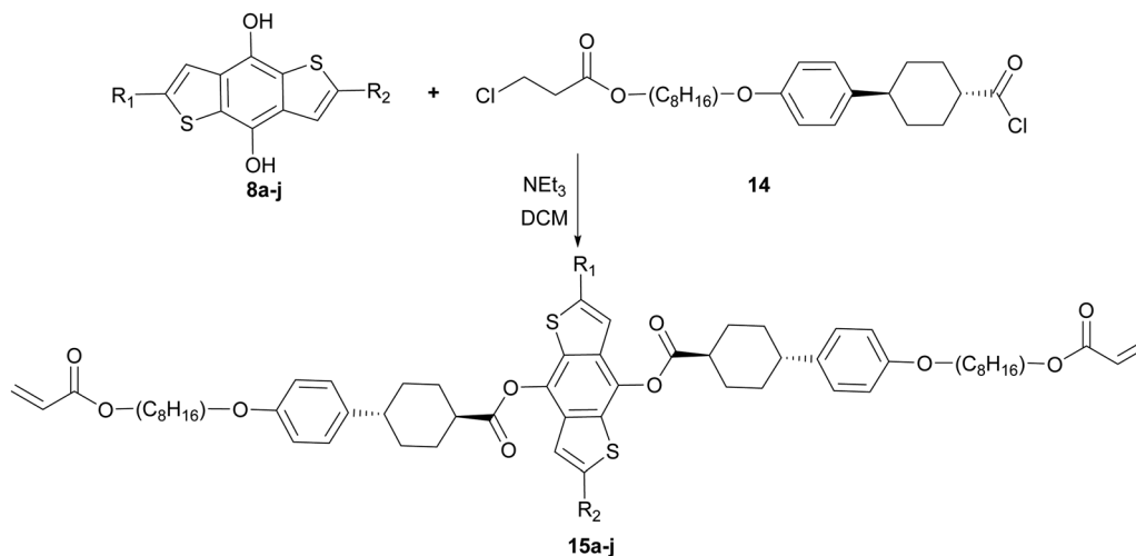
Scheme 5 Reaction scheme to give final product ( 15a–j ) where \text{R}_1 and \text{R}_2 are defined relative to the starting material described in Scheme 2.
