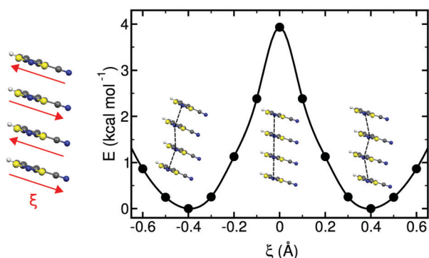
Fig. 16 Potential energy profile of an isolated stack of 4-NCBDDTA radicals along the reaction coordinate, \xi , defined in the left-most scheme. \xi describes a collective sliding motion of the radicals that preserves the inter-planar distance between them. The profile was computed with periodic boundary conditions along the stacking direction. The regular structure shown at \xi = 0 corresponds to the regular stack of the crystal structure at 300 K.
