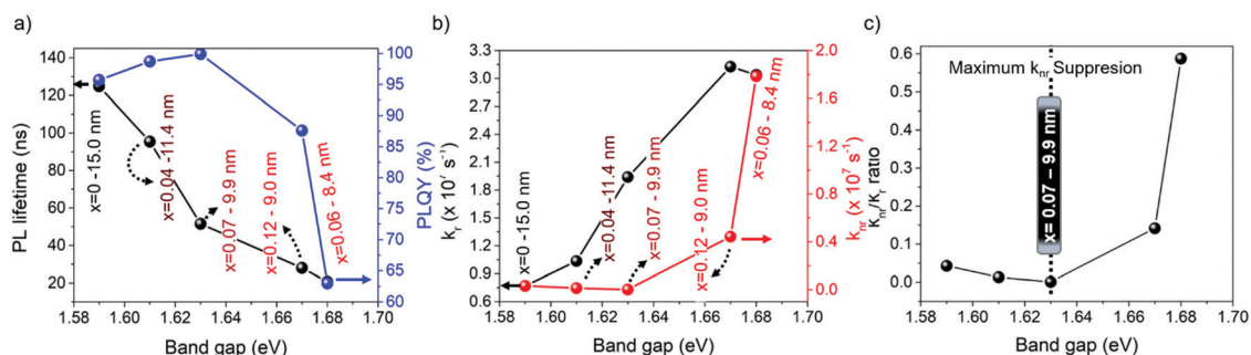
Fig. 5 (a) Behavior of the PL lifetime and PLQY, (b) radiative ( k_r ) and non-radiative recombination ( k_{\text{nr}} ) decay rate constants, and (c) their corresponding k_{\text{nr}}/k_r ratio for the FAPb 1-x Sr x I 3 PQDs colloidal solutions by varying the Sr fraction.
