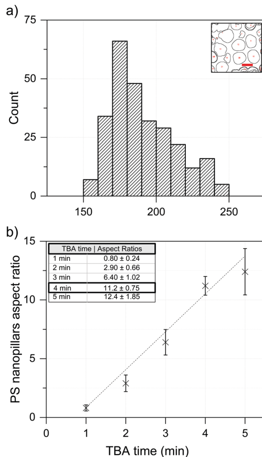
Fig. 2 (a) Size distribution histogram: average diameter of the polystyrene nanopillar = 185 \pm 22 \text{ nm} (inset: sample particle diameter analysis using the ImageJ software, scale bar = 200 nm). (b) Relationship between the aspect ratio of the PS nanopillars and the 80 °C TBA solvent contact time of the PDMS-coated AAO membranes: a longer TBA time led to a higher aspect ratio of the produced PS nanopillars (each data point is an average value with the standard deviation from 5 measurements).
