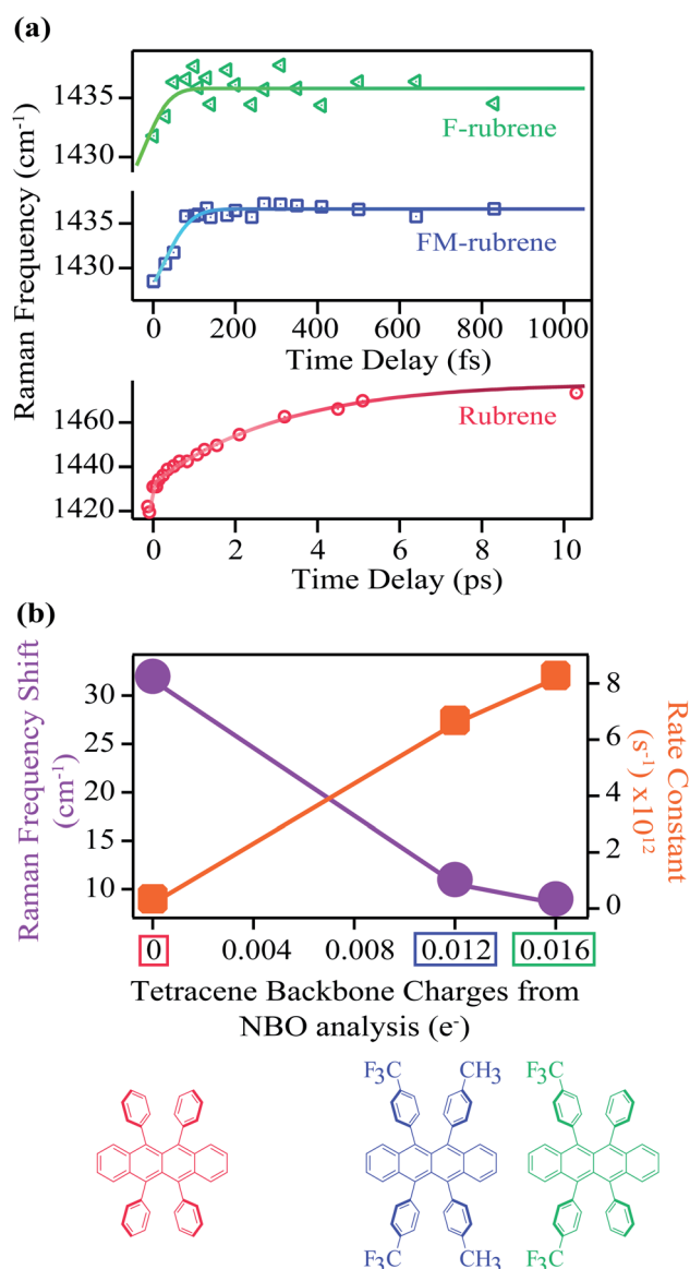
Fig. 3 (a) Transient Raman frequency evolution of the mode around 1430\text{ cm}^{-1} at time zero in crystalline rubrene, FM-rubrene and F-rubrene upon photoexcitation. Error bars are contained within the markers. (b) The corresponding total shift in the 1430\text{ cm}^{-1} Raman band position in the three molecules and the associated rate constants as a function of the total charge on the tetracene backbone from NBO population analysis.
