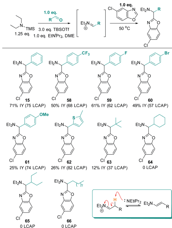
Scheme 16 Aldehyde scope. Conditions: azole (1.0 eq.), TBSOTf (0.416 mL, 1.813 mmol, 3.0 eq.), TMS- \text{NEt}_2 (1.25 eq.), PhCHO (1.0 equiv.), \text{EtNPr}_2 (1.0 equiv.), \text{N}_2 , 50 °C, 18 h.
