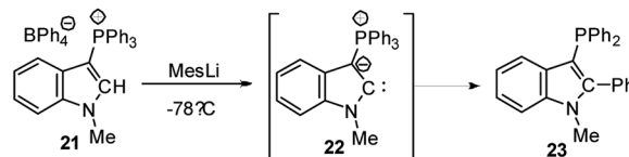
Scheme 3 Attempted isolations of CAYC 22 .
