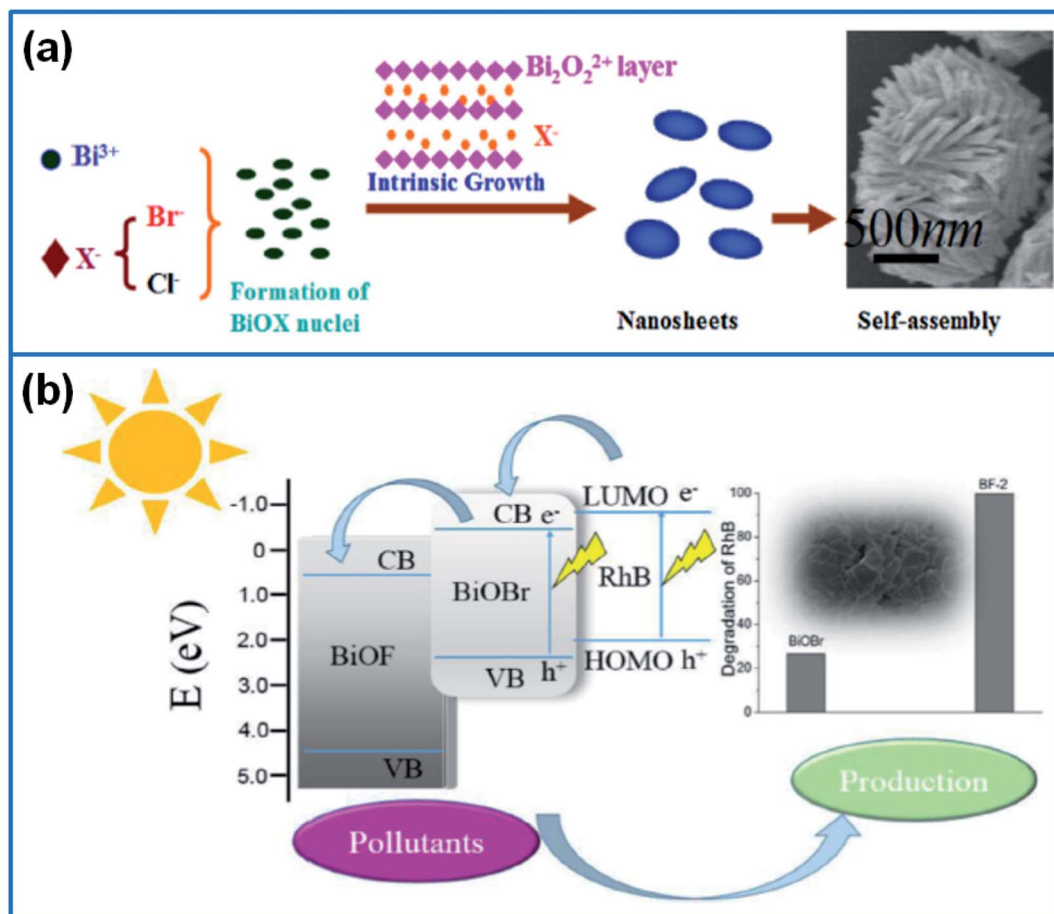
Fig. 7 (a) Schematic illustration for fabricating BiOCl/BiOBr microsphere. 127 Copyright 2018 Elsevier. (b) Schematic illustration of the charge transfer and separation of BiOBr/BiOF heterojunction. 130 Copyright 2017 Elsevier.
