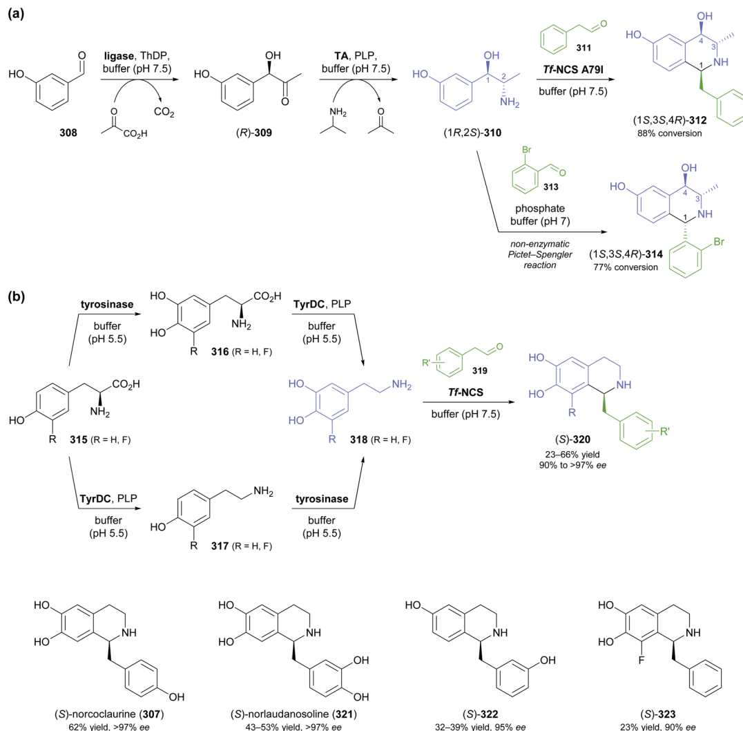
Scheme 40 In situ formation of amine substrates for norcoclaurine synthase: (a) combination of biocatalytic carbonylation and transamination leads to metamaminol (310), which can undergo enzymatic or phosphate-catalysed Pictet–Spengler reactions. (b) Tyrosinase and tyrosine decarboxylase (TyrDC) can be used to prepare dopamine and its derivatives from the corresponding amino acids.
