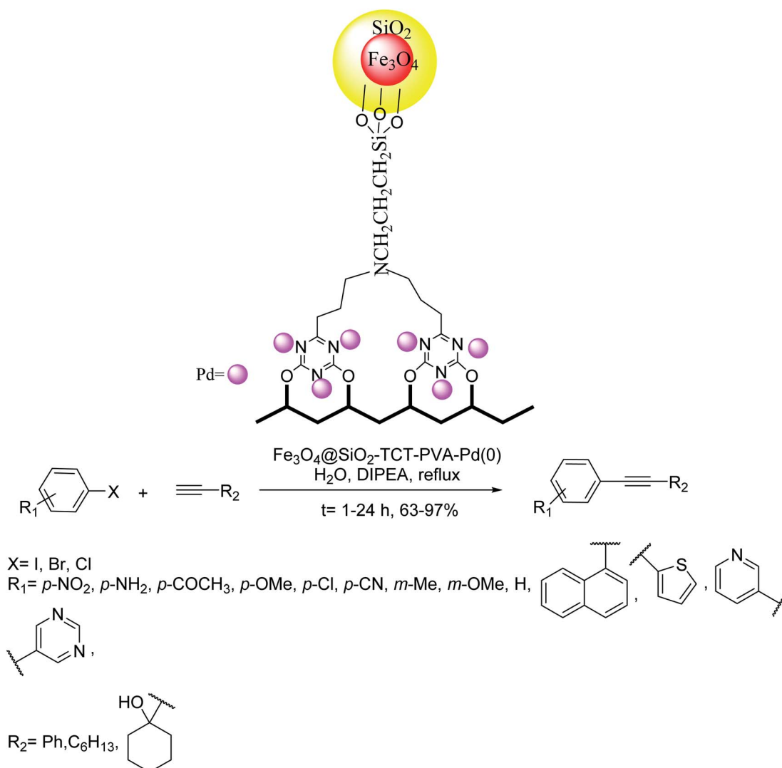
Scheme 35 Copper-free Sonogashira coupling reactions in the presence of the magnetic silane- 2,4,6-trichloro-1,3,5-triazine-polyvinyl alcohol-palladium ( \text{Fe}_3\text{O}_4@ \text{SiO}_2\text{-TCT-PVA-Pd}(0) ).
