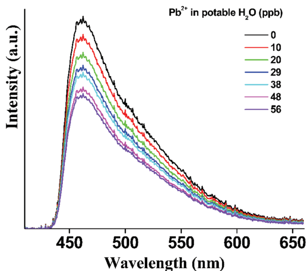
Fig. 9 The fluorescence titration ( \lambda_{\text{exc}} = 380 nm) of a stirred suspension of p-UCR-20 in water ( 0.1 \text{ mg mL}^{-1} ) upon the addition of aliquots from a \text{Pb}^{2+} standard stock solution (concentration = 1000 ppb) in potable water.
