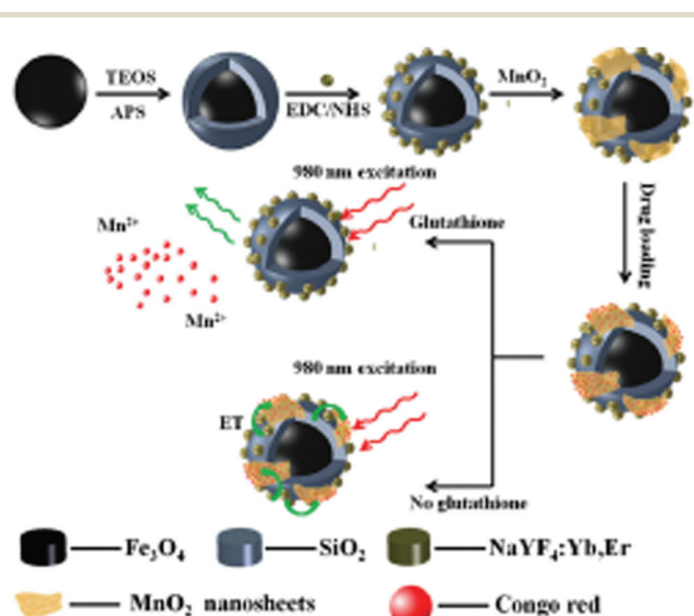
Fig. 1 Schematic illustration of the synthetic procedure for the preparation of the MSU/MnO 2 –CR drug delivery system. Reprinted with permission from ref. 122 Zhao et al. , Dalton Trans. , 2014, 43, 451–457. Copyright©2014, The Royal Society of Chemistry.
