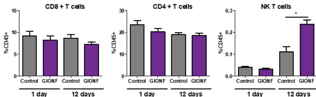
Fig. 3 Changes in the lymphoid subset in the spleen 1 day and 12 days after GIONF exposure. Results are shown as mean \pm SEM of n = 5 –6 per condition. T-Student, Mann–Whitney (control vs. GIONF in each time point) * p -value < 0.05 .
