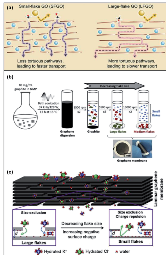
Fig. 7 (a) Intercalation of \text{La}^{3+} (blue sphere) onto the nanosheets allowing permeation of methanol (C, black; H, white; O, red) but not other solute molecules (yellow sphere). As compared to SFGO, using LFGO makes the methanol molecule pass through a more tortuous and longer pathway, which causes lower methanol permeance. Adapted with permission from ref. 73. American Association for the Advancement of Science, copyright 2020. (b) A schematic illustration to depict the synthesis of graphene dispersions to decrease the flake size using bath sonication. (c) An illustration to demonstrate the combination of size exclusion and ionic charge repulsion utilised in SFGO as compared to LFGO when substances permeate through. Adapted with permission from ref. 74. Elsevier Science Ltd, copyright 2019.
