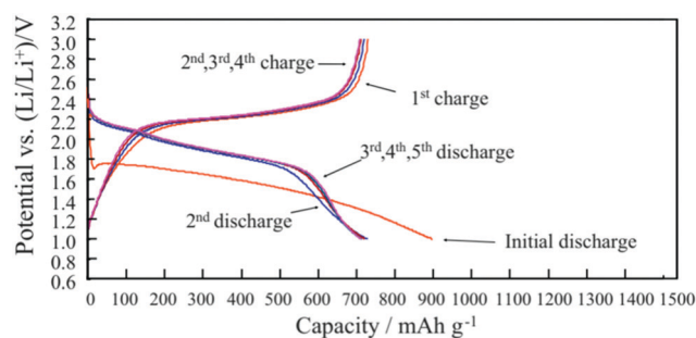
Fig. 2 Charge/discharge performance of SPAN cathode in 1 M \text{LiPF}_6/\text{EC} + \text{DEC} . Image reprinted with the permission from ref. 49. Copyright © 2012, Elsevier License 5041181200155.
