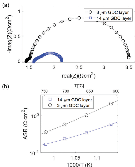
Fig. 7 (a) Impedance spectra of symmetrical cells with 3 and 14 \mu\text{m} GDC layer thickness tested at 600 °C in 7% CO in \text{CO}_2 atmosphere. (b) Arrhenius plot of the ASR.
