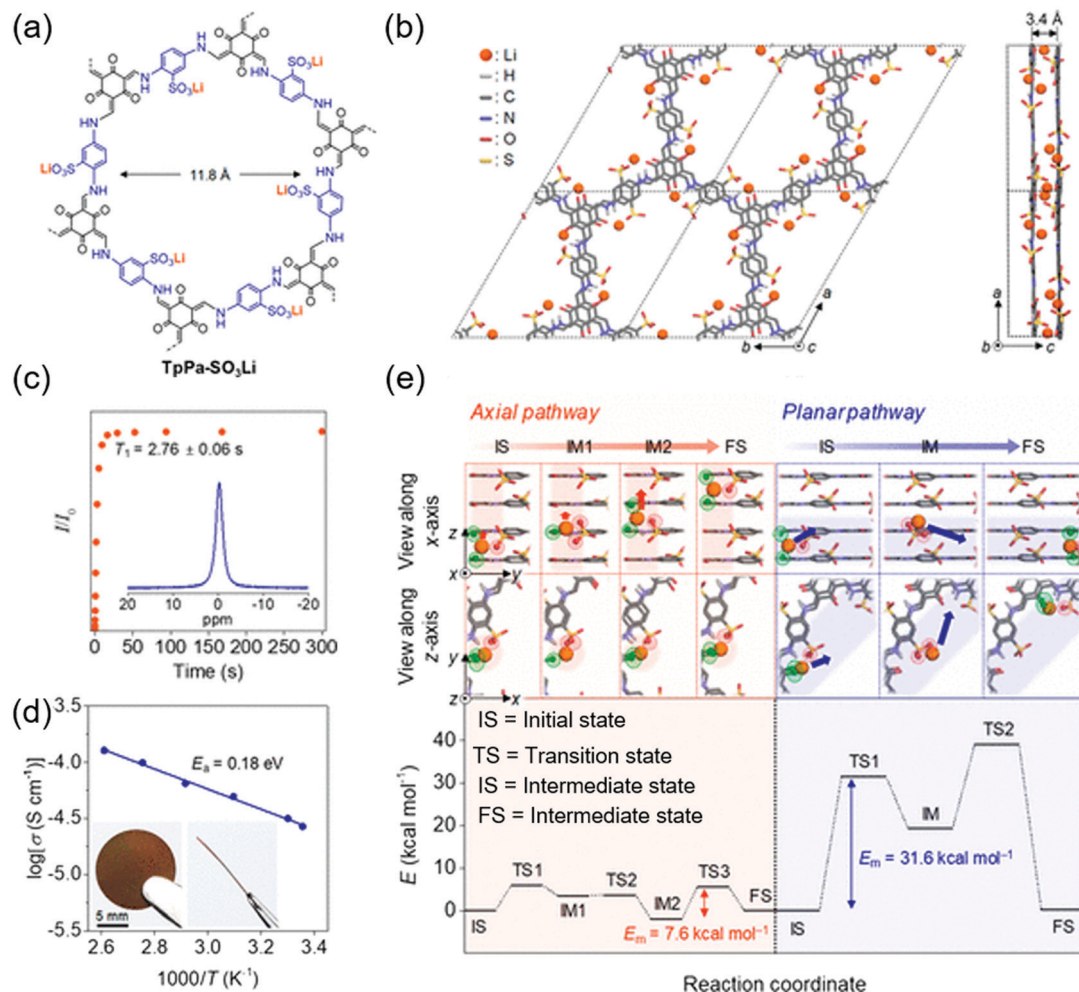
Fig. 22 Solvent-less, single Li-ion conduction in COFs. (a) Chemical structure of lithiated COF for \text{Li}^+ conduction. (b) Simulated structure of TpPa- \text{SO}_3\text{Li} along c - and b -axes. (c) Saturation recovery plot (for complete lithiation of COF) from ^7\text{Li} MAS NMR spectra. (d) Calculation of activation energy ( E_a ) for Li-CON-TFSI in hydrous conditions by the methods of Arrhenius. (e) Depiction of \text{Li}^+ migration inside the pore through axial or planar pathway. Reproduced with permission. 160 Copyright 2019, American Chemical Society.
