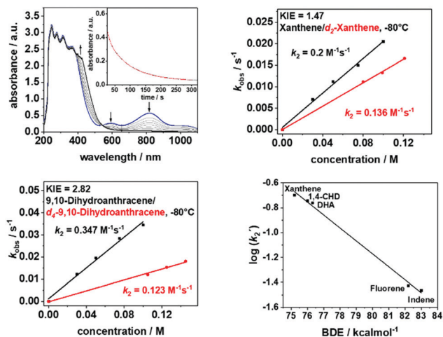
Fig. 3 Top left: Changes in the UV-Vis-spectra of a 1 mM solution of 1-trans in \text{CH}_2\text{Cl}_2/\text{CH}_3\text{CN} (95:5) at -80\text{ }^\circ\text{C} upon addition of 100 eq xanthene; the inset shows the time trace for the decay of the 815 nm band and its pseudo-first order fit; top right: plots of the pseudo-first order rate constants k_{\text{obs}} vs. the substrate concentrations for xanthene and d_2 -xanthene in order to determine the kinetic isotopic effect (KIE) for the reaction of 1-trans with xanthene; bottom left: plots of the pseudo-first order rate constants k_{\text{obs}} vs. the substrate concentrations for 9,10-dihydroanthracene (DHA) and d_4 -DHA in order to determine the kinetic isotopic effect (KIE) for the reaction of 1-trans with DHA; bottom right: plot of the logarithms of the second-order rate constants k_2' vs. the C-H BDEs of the substrates with 1-trans in \text{CH}_2\text{Cl}_2/\text{CH}_3\text{CN} (95:5).
