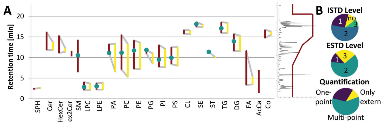
Fig. 4 Application of LILY with RP-LC and its benefits. (A) Broad RT coverage: the RT coverage for different lipid classes (each polygon corresponds to one lipid class) is shown, the left red side of the polygon shows the elution range (1st to last eluting lipid of each class) of human plasma lipids, the right yellow side shows the elution range of LILY lipids, lipid classes shown as the vertical line are only present in plasma, and green dots show the elution time of the deuterated single-lipid-per-class mixture SPLASH® LIPIDOMIX® Mass Spec Standard. A total ion chromatogram and the gradient starting at 55% B and going up to 100% B are shown on the right side as visual help. (B) Distribution of the used ISTD, quantification strategies and the ESTD. ISTD: 80% of analytes have RT-matched ISTD; the level (defined by LSI) 30 of the ISTD is shown. Quantification strategies: 59% of analytes are quantified via multi-point calibration; three different quantification strategies have been applied: multi-point, external multi-point calibration with internal standardization; one-point, surrogate internal standardization without external standardization; only external, multi-point calibration without the use of the ISTD and ESTD; 12% of analytes are available as the ESTD and 63% have co-ionized ESTD.
