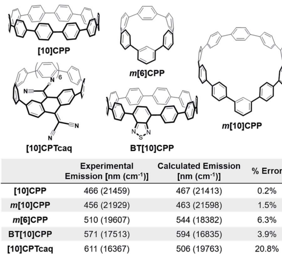
Fig. 2 Experimental and calculated fluorescence and associated error of [10]CPP, m[10]CPP, m[6]CPP, BT[10]CPP, and [10]CPTcaq. Error calculated in cm -1 .
