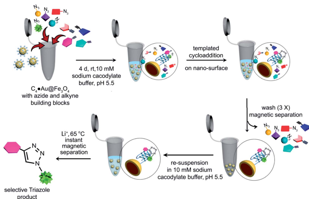
Fig. 4 Schematic representation of the target guided synthetic approach using i-motif magnetic nanotemplates ( c-MYC \text{C}_4\cdot\text{Au@Fe}_3\text{O}_4 & BCL2 \text{C}_4\cdot\text{Au@Fe}_3\text{O}_4 ) for in situ formation of potent binders.
