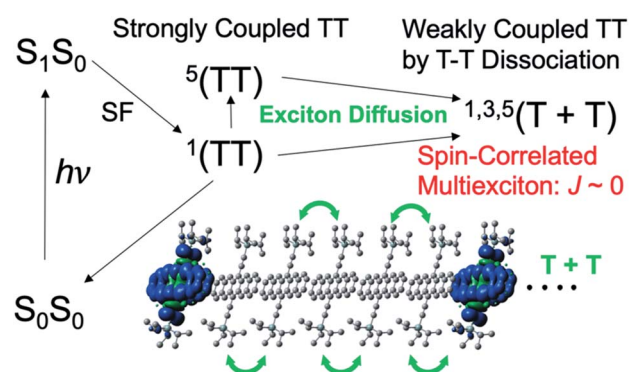
Fig. 1 Schematic representation of the spin-correlated triplet pair (SCTP) state of ^{1,3,5}(T + T) generated by the SF in thin films of TIPS-Pn by the triplet energy transfer via the TT state.
