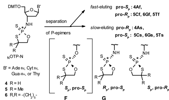
Scheme 2 Effects of silica gel separation of P-diastereomers of 2-thio-1,3,2-oxathiaphospholane monomers 4-6 . The descriptors pro-R_P and pro-S_P indicate the absolute configuration of P-atom in the subsequently formed internucleotide phosphoramidothioate linkages. The structure F is given only for comparison with G.
